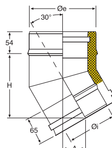
Coude 30°
