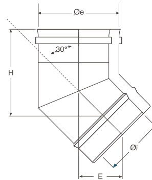
Coude 30°
