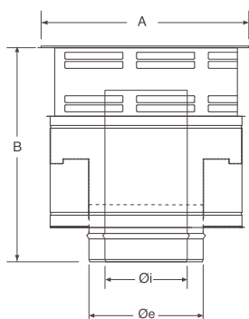
Terminal vertical
