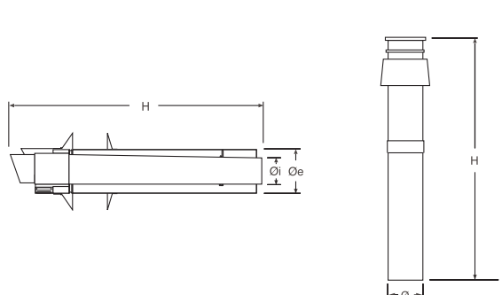
Terminal horizontal
