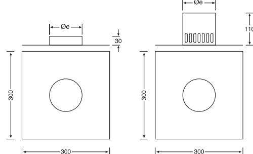
Plaque type C9
